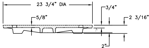
COVER SECTION
