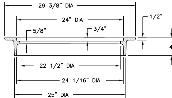
FRAME SECTION
